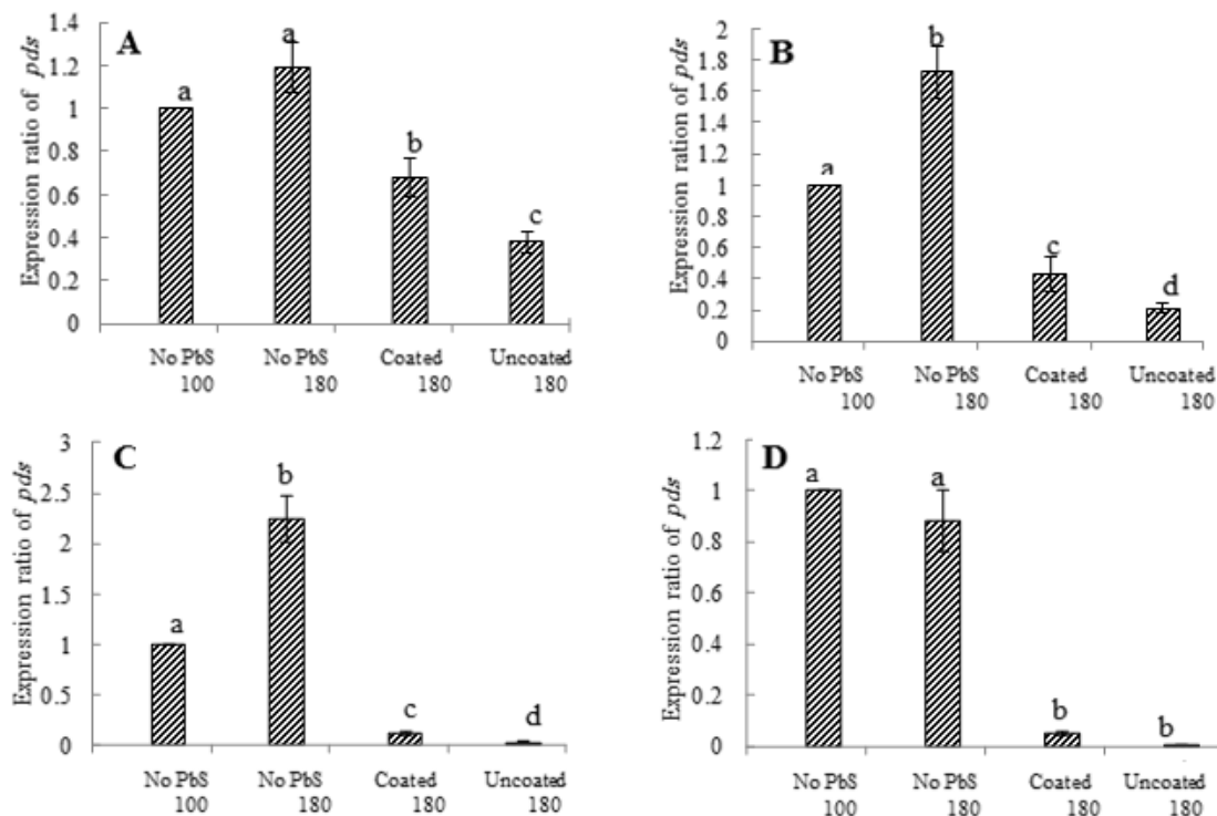
Figure 1: Effects of uncoated and gum-Arabic coated lead sulfide nanoparticles (GA-coated PbS NPs) and light intensity on mRNA levels of phytoene desaturase ( Pds ) in Dunaliella salina Teod. Cells grown at 100 \mu\text{mol photons m}^{-2} \text{s}^{-1} light intensity with no PbS NPs (control culture) were transferred to 180 \mu\text{mol photons m}^{-2} \text{s}^{-1} intensity and exposed to PbS NPs. Samples were taken at 3 h (Box A), 6 h (Box B), 12 h (Box C) and 48 h (Box D) after shift to higher light intensity for mRNA analysis.
