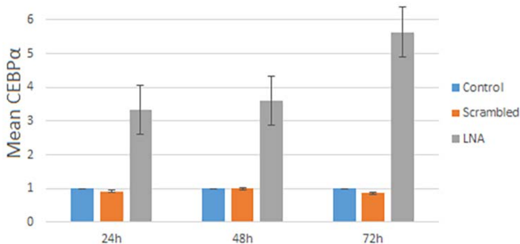
Figure 3: Expression level of CEBP \alpha by qRT PCR at 24, 48 and 72 h after transfection; data analysis performed by the \Delta\Delta C_t method and untreated group (control) was considered as a reference. Data are mean \pm S.D. of triple independent experiments. P < 0.021 .
