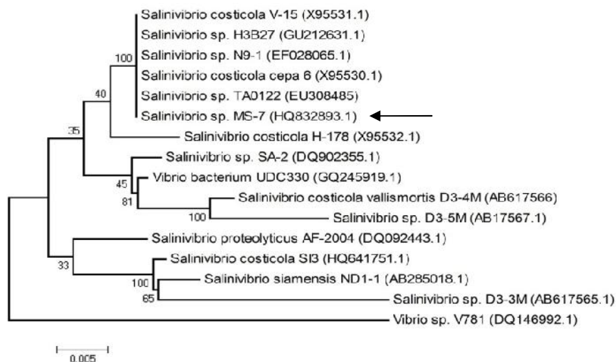
Figure 2: Phylogenetic tree showing the taxonomic position of isolate Salinivibrio sp. strain MS-7 and relationships between strain MS-7, species of the genus Salinivibrio and related taxa based on 16S rRNA gene sequences. The branching pattern was generated by the neighbour-joining method
