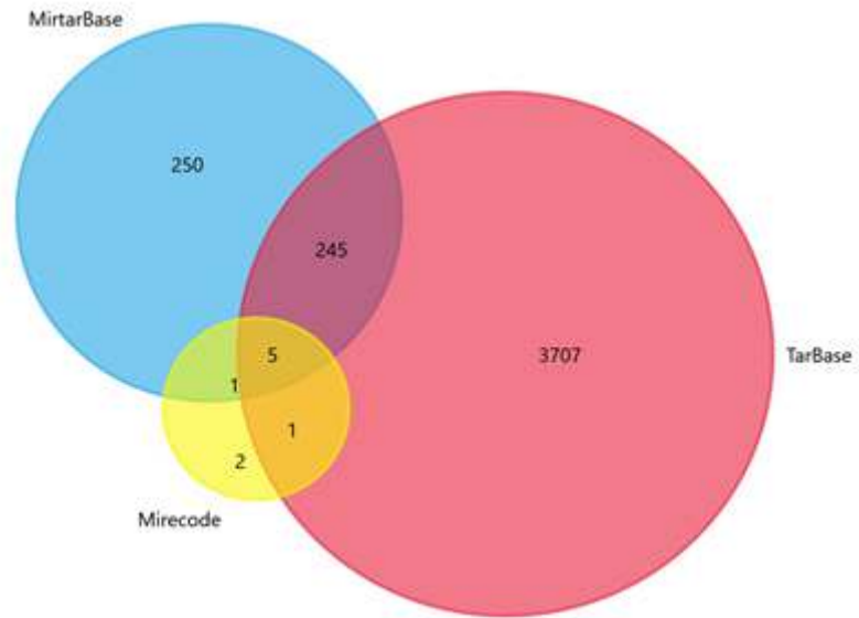
Figure S1: Venn diagram shows that 245 genes were overlapped between 3 different databases
